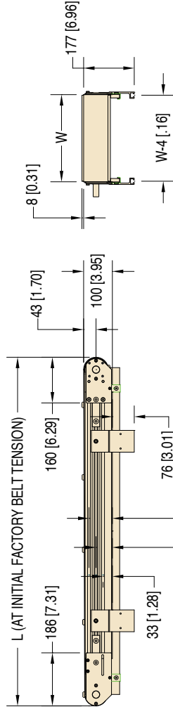
FIXTURED BELT
