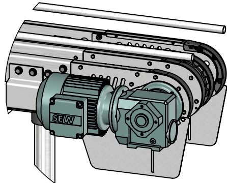
Direct Drive
