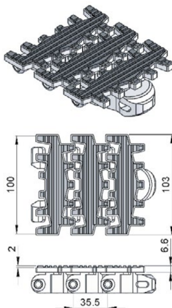
Friction Top Chain FCFT-5B
