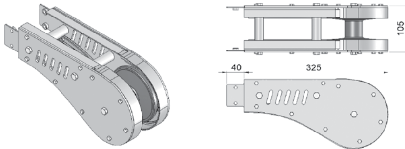
SC Idler End-A105
