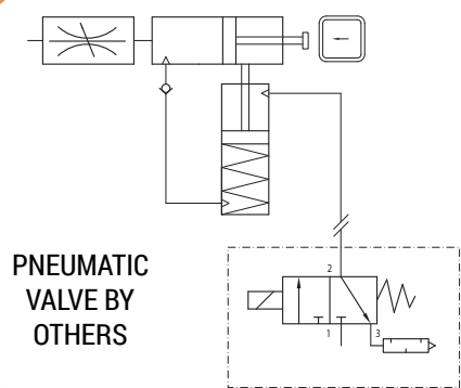
PNEUMATIC SCHEMATIC
