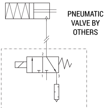
PNEUMATIC SCHEMATIC
