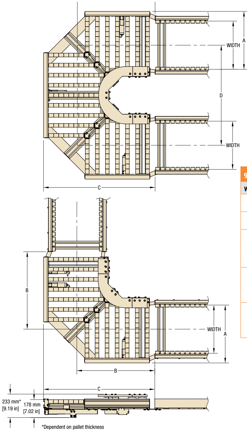
ERT250: 90 Degree Corner Conveyor
