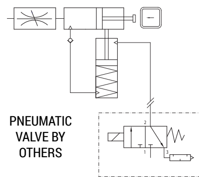
PNEUMATIC SCHEMATIC
