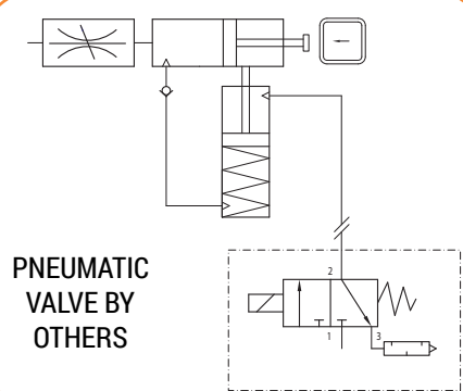
PNEUMATIC SCHEMATIC
