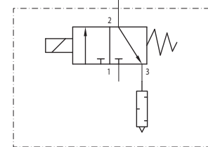
PNEUMATIC SCHEMATIC
