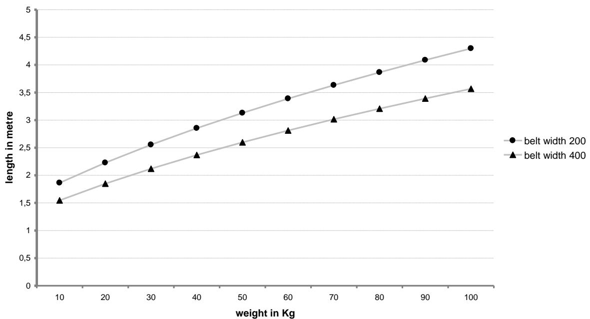
Figure 4-11: Maximum weight at end of conveyor with supports on wheels
