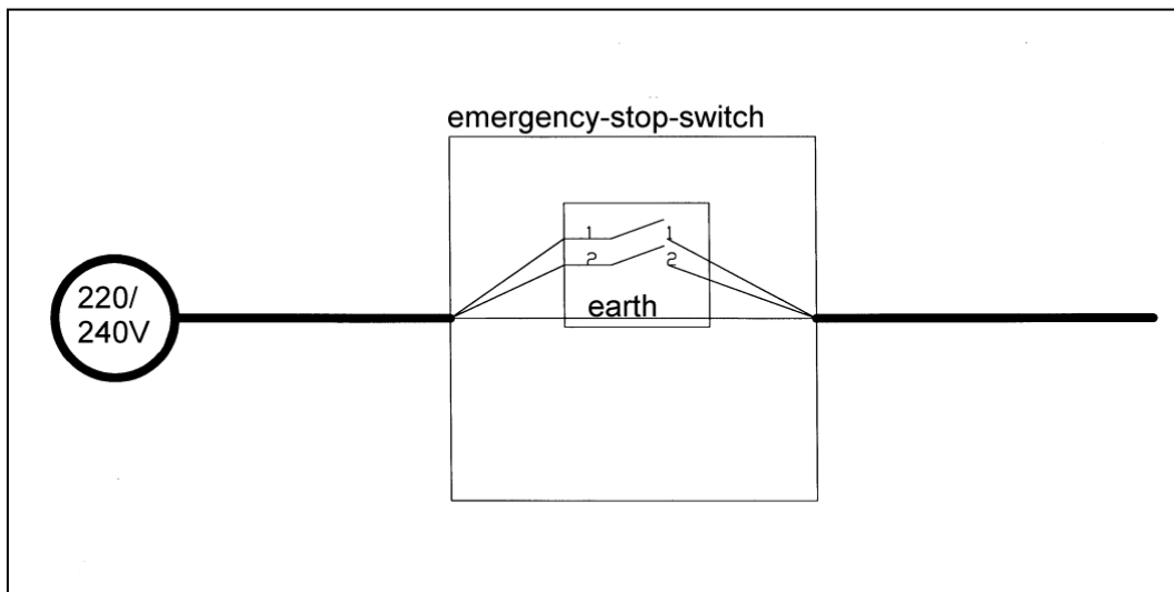
Figure 3-10: Connection of emergency-stop-switch to 230V 50Hz
