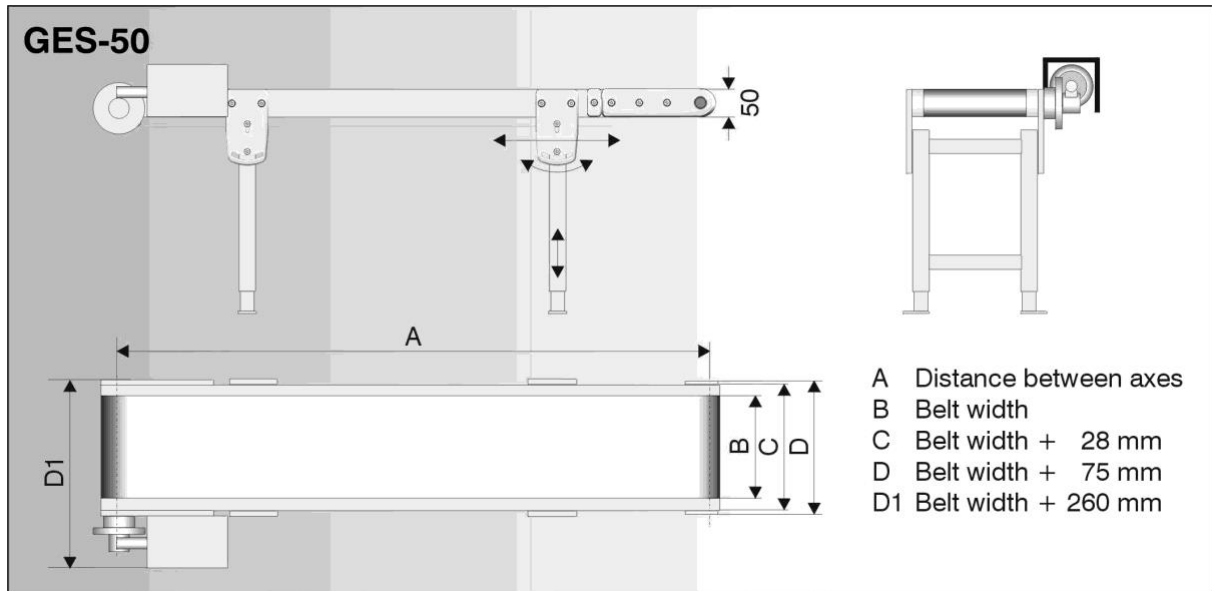
Figure 3-1: Basic dimensions GES-50
