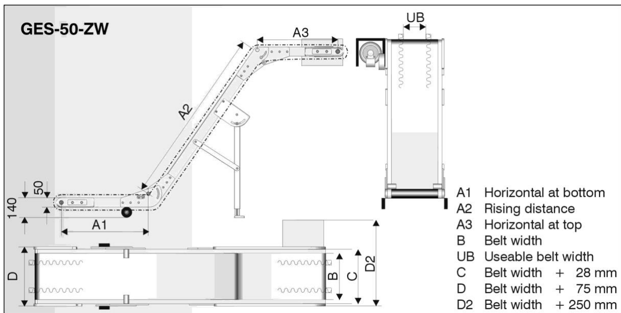
Figure 3-3: Basic dimensions GES-50-ZW
