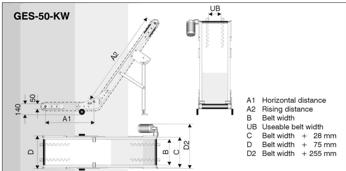
Figure 3-2: Basic dimensions GES-50-KW
