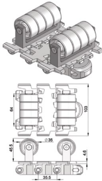
Roller Cleat Chain FCRC-5B-L#
