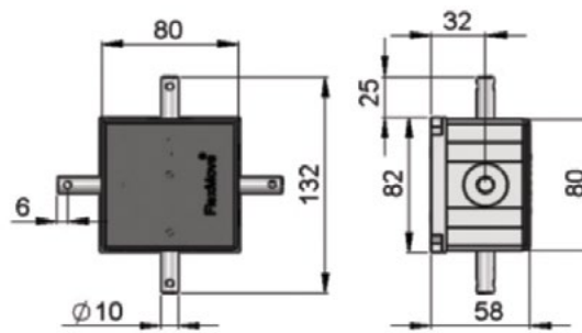
FZGB-904 Angle Gear Unit – 4 direction
