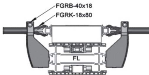
Width & Height Adjustable Guide Rail Assembly
