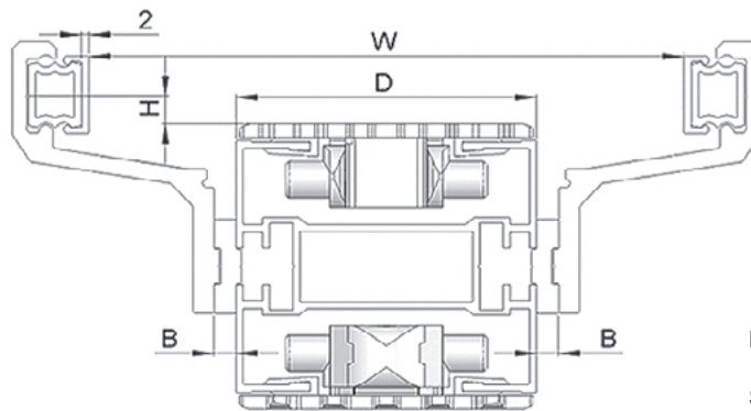
FGRB-53x42 Assembly
