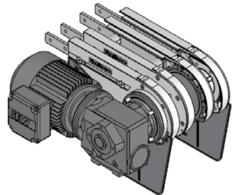
FU Direct End Drive with Motor (RIGHT) FUDD-A180-XDY (See Chart)
