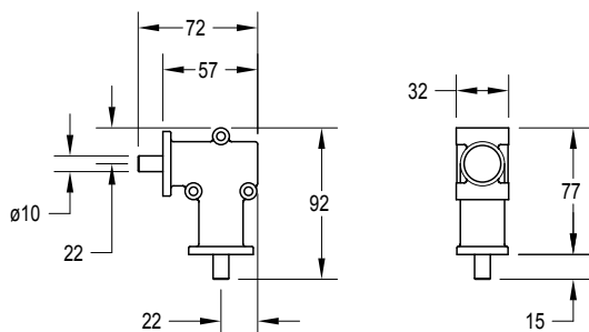
807-3635 90° Gearbox
