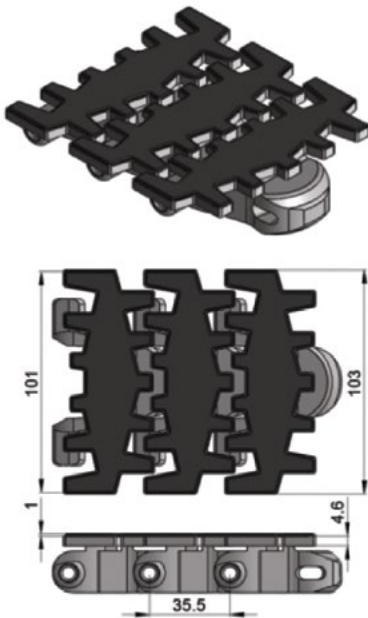
Friction Top Chain FCFT-5A
