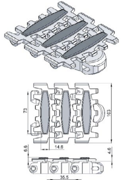
Friction Top Chain FCFT-5
