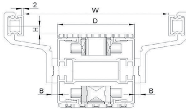
FGRB-49x42 Assembly
