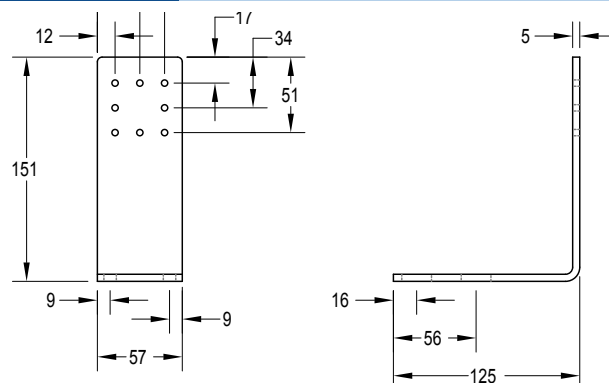
75164386 90° Gearbox Mount
