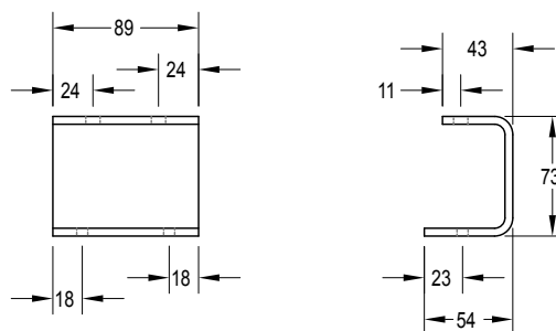
75148092 Conveyor Gearbox Mount
