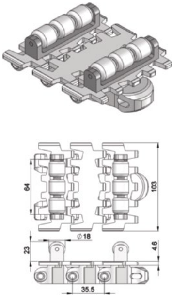
Roller Cleat Chain FCRC-5A-L#
