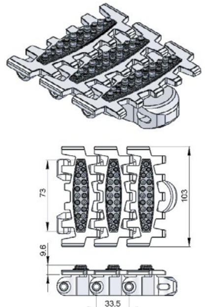
Friction Top Chain FCFT-5C
