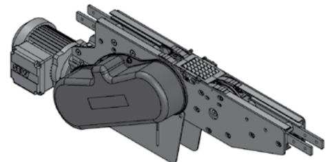
FS Combined Suspended Drive & Idler (RIGHT)
