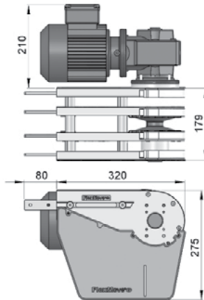
FU Direct End Drive with Motor (LEFT) FUDD-A180-XDY (See Chart)
