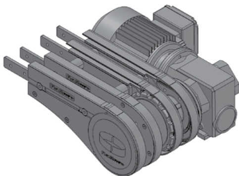
FU Direct End Drive unit without Motor GP (LEFT) FUDD-A180GP-XDY (See Chart)
