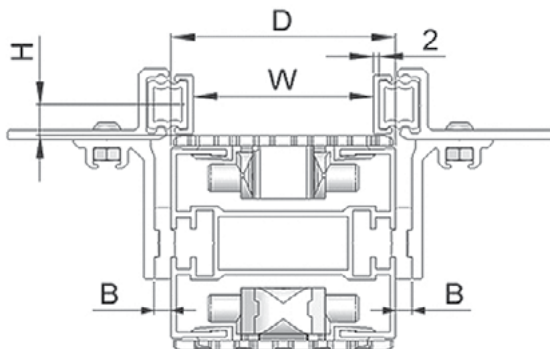
FGRA-8x39x45 Assembly
