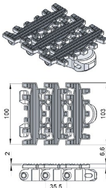
Friction Top Chain FCFT-5B
