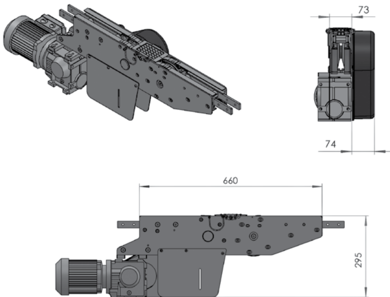
FS Combined Suspended Drive & Idler (LEFT)
