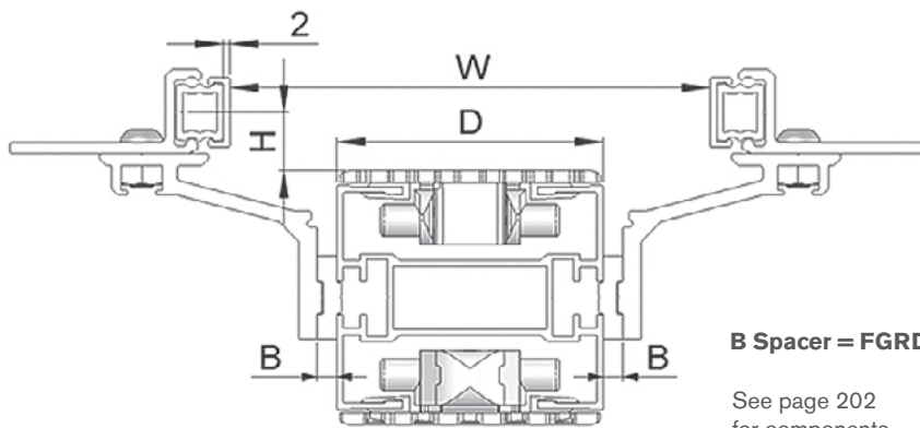
FGRA-26x39x45 Assembly
